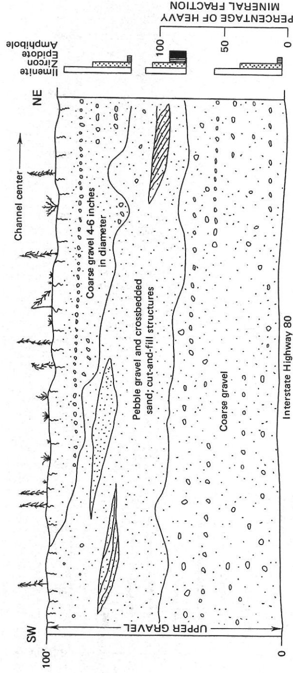
FIGURE 24.—Tertiary gravel (upper gravel) exposed along Interstate Highway 80 near Gold Run. Heavy minerals shown at right.
