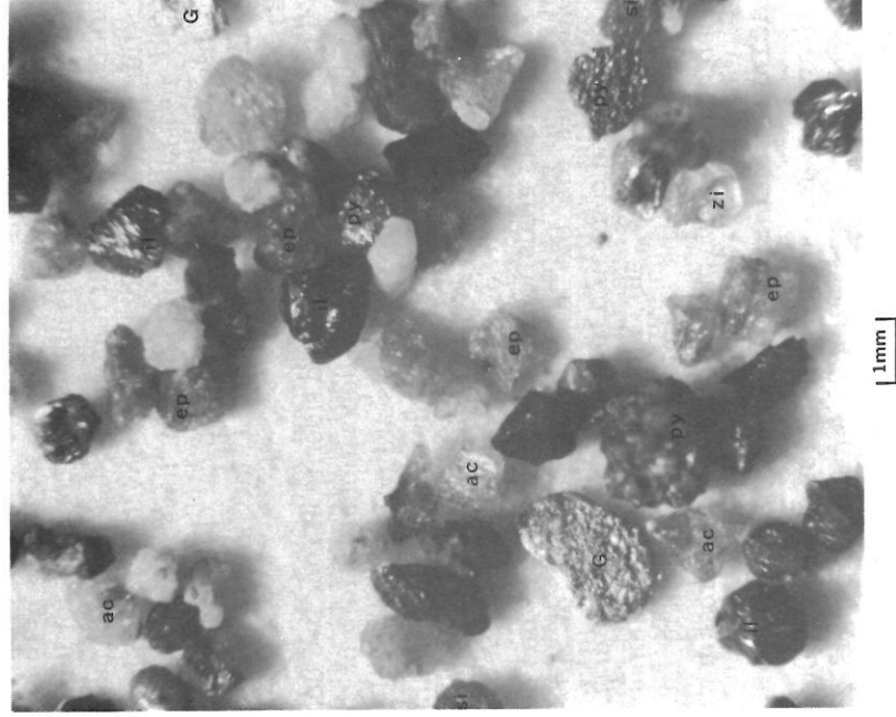
FIGURE 22.—Heavy minerals from lower gravel of hole A in the North Columbia Diggings. Samples collected from a depth of 365 feet. zi, zircon; il, ilmenite; py, pyrite; si, siderite; ep, epidote; ac, actinolite; G, gold.
