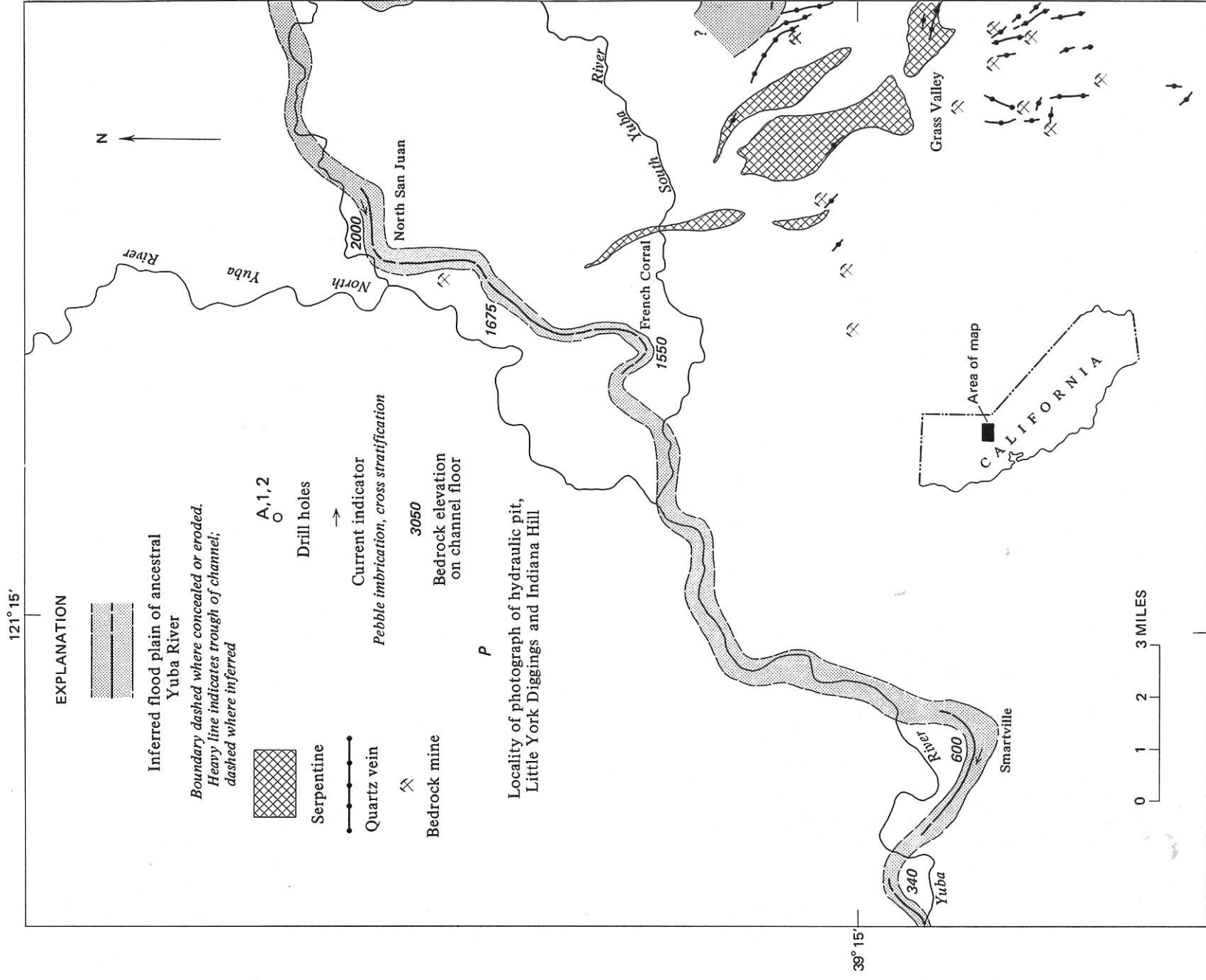
FIGURE 2.—Trace of part of ancestral Yuba River
