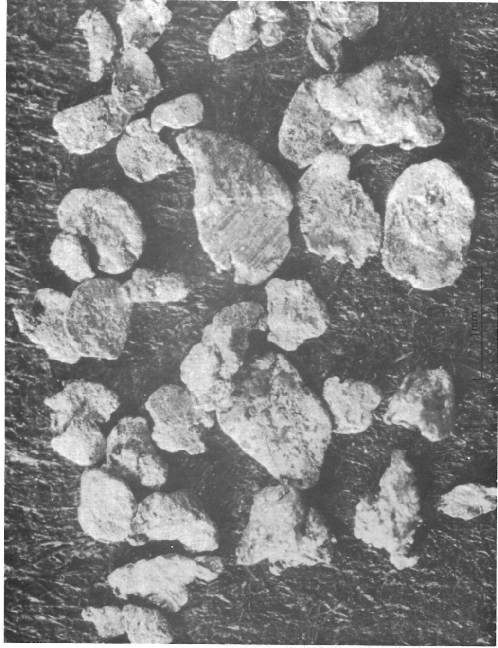
FIGURE 19.—Typical placer gold derived from lower gravel in North Columbia hydraulic pit.
